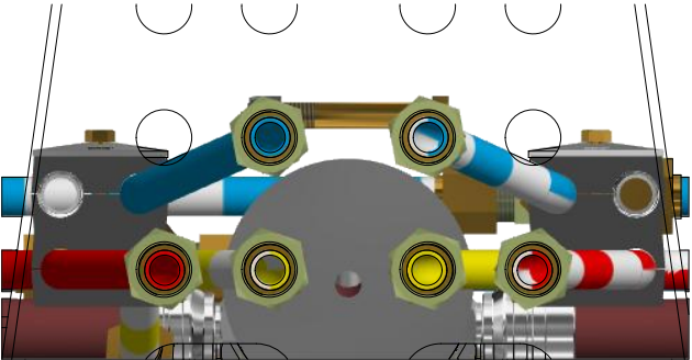
HOSE ALIGNMENT AT BULKHEAD
